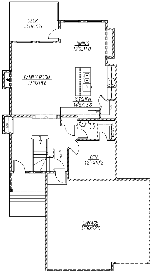
MAIN FLOOR PLAN-1113 SQ.FT.
