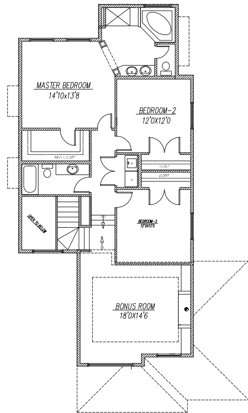
UPPER FLOOR PLAN-1282 SQ.FT.
