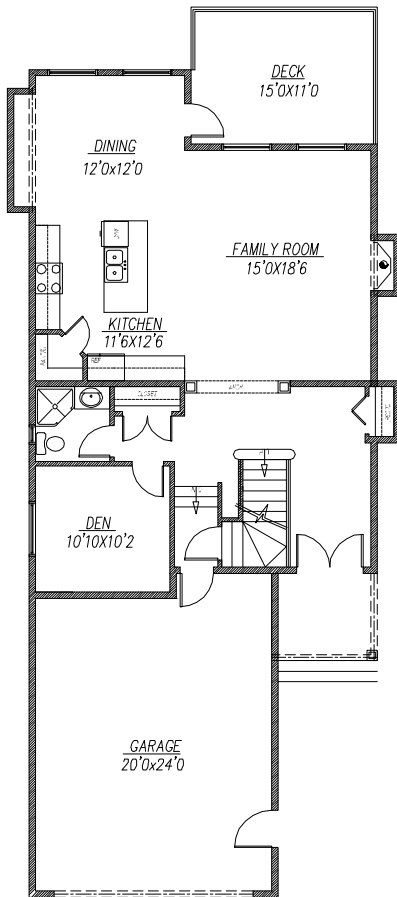
MAIN FLOOR PLAN-1103 SQ.FT.
