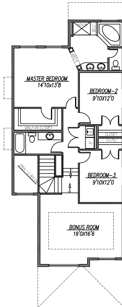
UPPER FLOOR PLAN 1184 SQ.FT.
