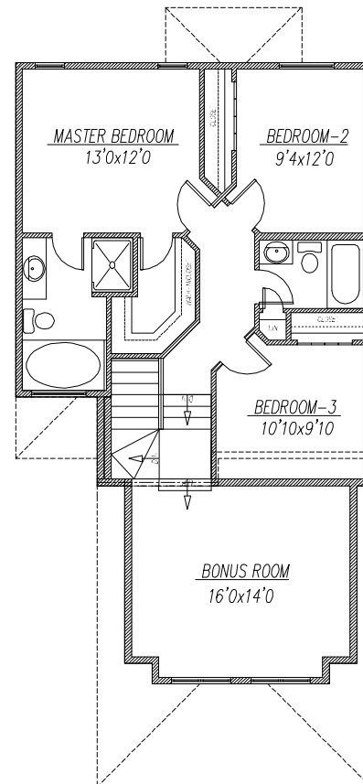
UPPER FLOOR PLAN-946 SQ.FT.
