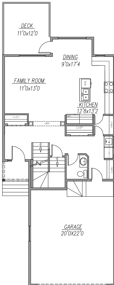
MAIN FLOOR PLAN-785 SQ.FT.
