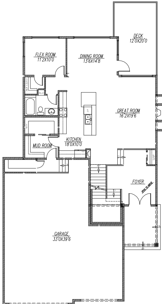
MAIN FLOOR PLAN-1419 SQ.FT.
