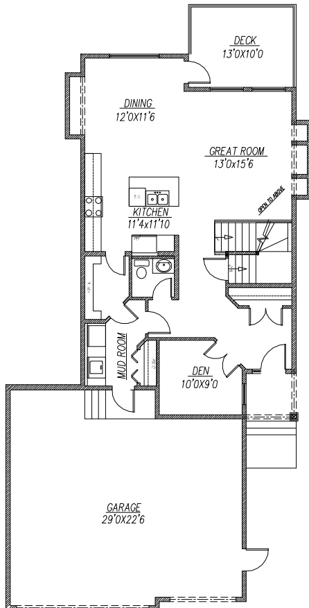
MAIN FLOOR PLAN-1060 SQ.FT.
