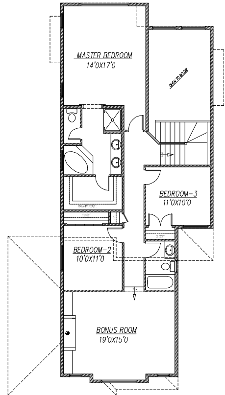
UPPER FLOOR PLAN-1223 SQ.FT.
