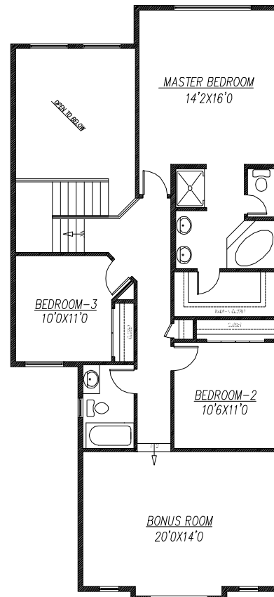
UPPER FLOOR PLAN-1239 SQ.FT.
