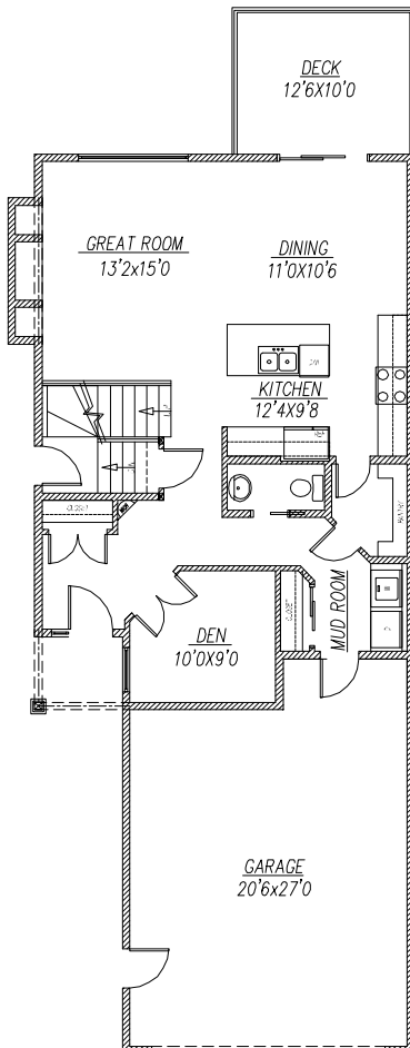
MAIN FLOOR PLAN-945 SQ.FT.
