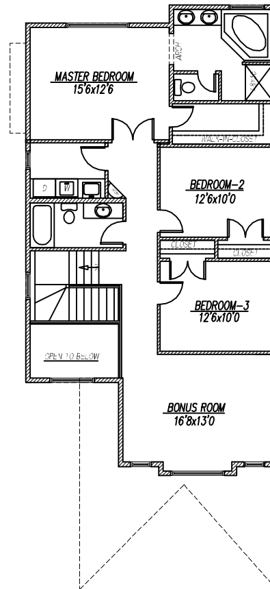
UPPER FLOOR PLAN 1175 SQ.FT.
