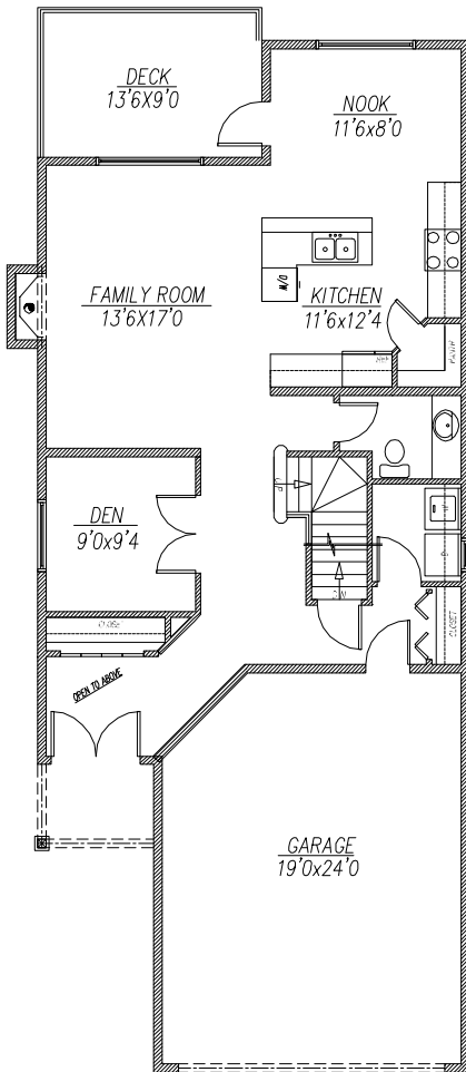
MAIN FLOOR PLAN-957 SQ.FT.
